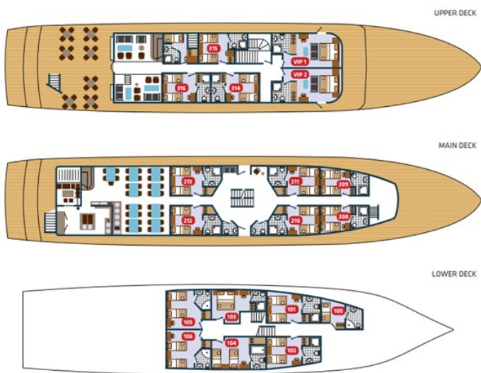
Main Deck
